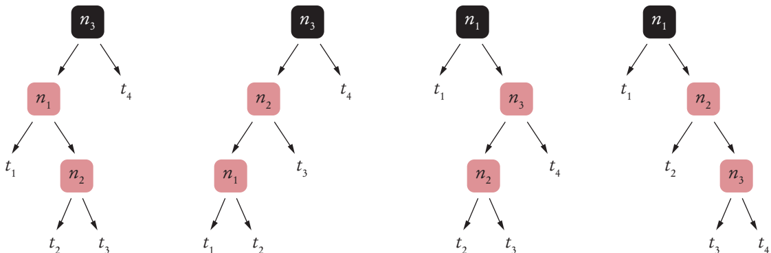
Figure 21 The Four Possible Configurations of a “Double Red”
