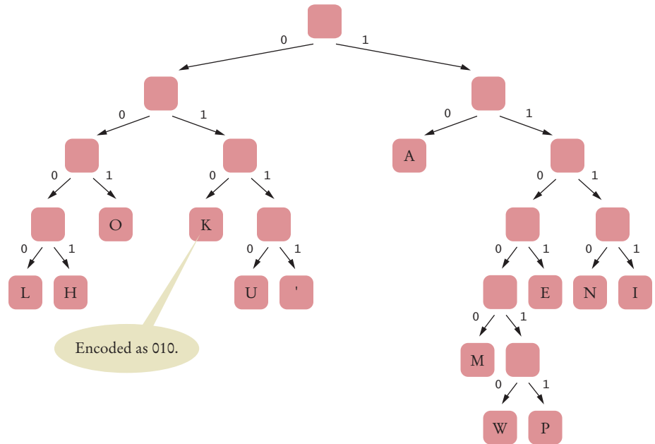
Figure 5 A Huffman Tree for Encoding the Thirteen Characters of Hawaiian Text
