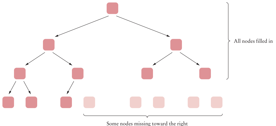
Figure 26 An Almost Completely Filled Tree
