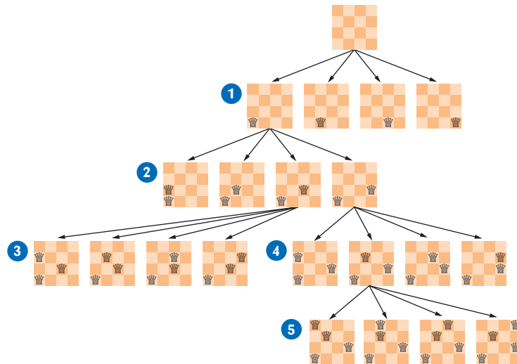
Figure 6 Backtracking in the Four Queens Problem
