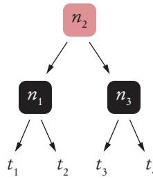
Figure 22 Fixing the “Double Red” Violation
