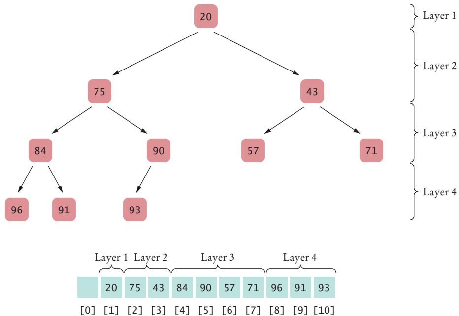
Figure 30 Storing a Heap in an Array
