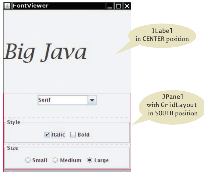
Figure 9 The Components of the FontFrame
