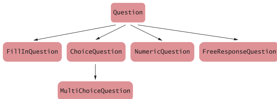
Figure 3 An Inheritance Tree
