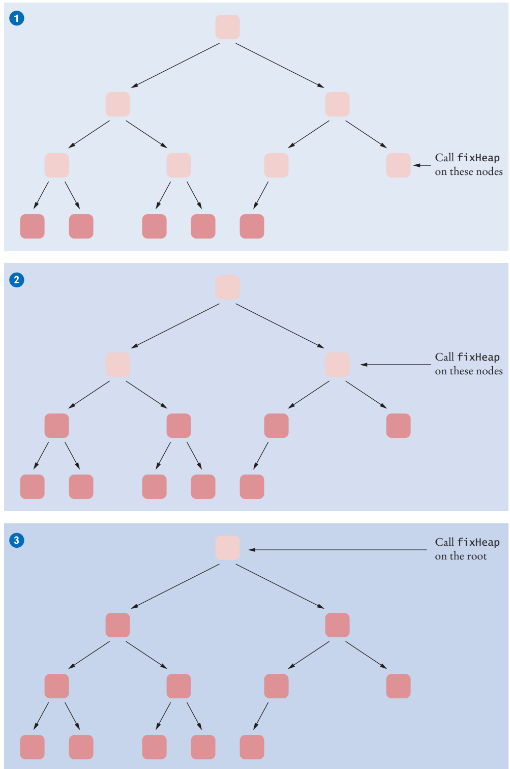
Figure 31 Turning a Tree into a Heap
