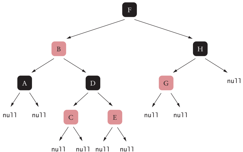
Figure 18 A Red-Black Tree
