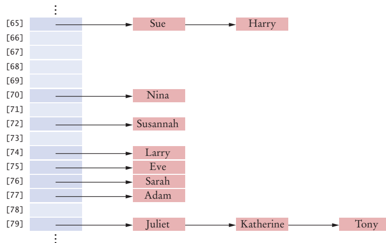
Figure 15 A Hash Table with Buckets to Store Elements with the Same Hash Code
