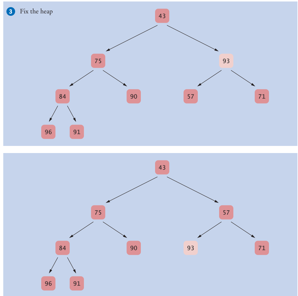
Figure 29 (continued) Removing the Minimum Value from a Heap
