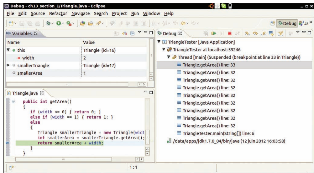
Figure 1 Debugging a Recursive Method
