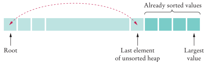
Figure 32 Using Heapsort to Sort an Array
