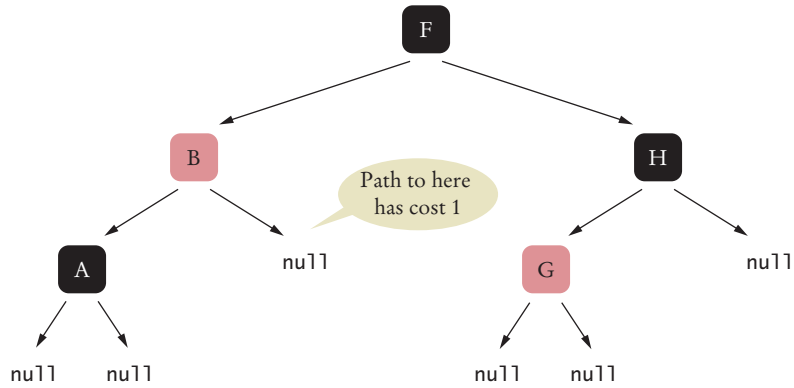
Figure 19 A Tree that Violates the “Equal Exit Cost” Rule
