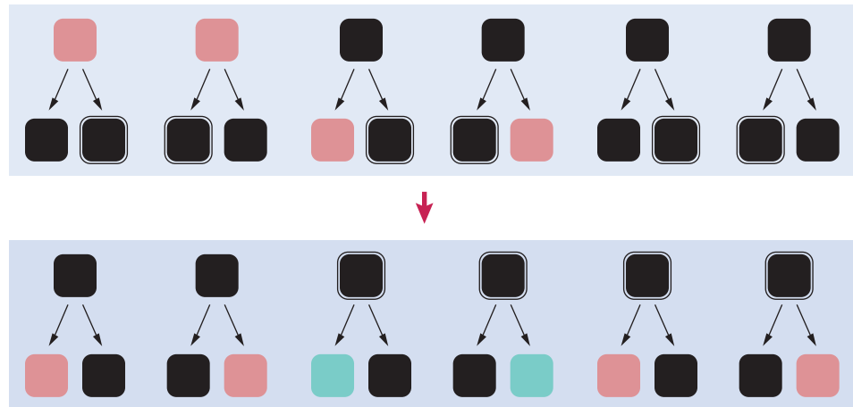
Figure 25 Bubbling Up a Double-Black Node
