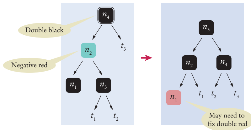
Figure 23 Eliminating a Negative-Red Node with a Double-Black Parent
