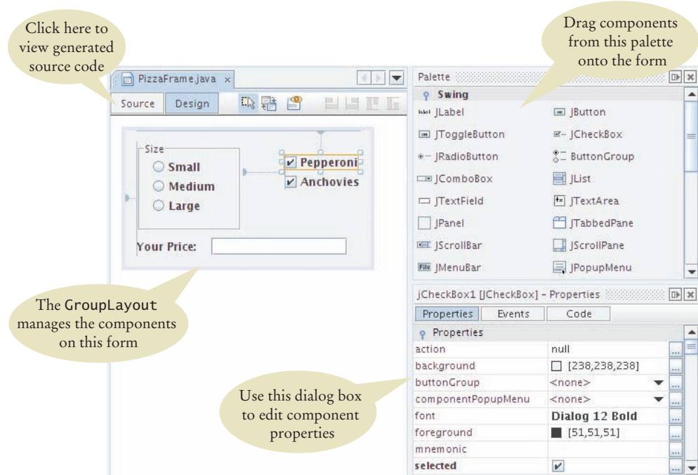
Figure 10 A GUI Builder
