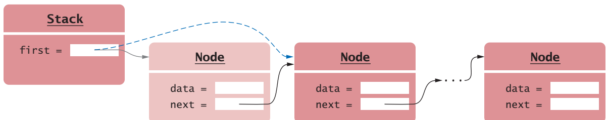
Figure 10 Push and Pop for a Stack Implemented as a Linked List
