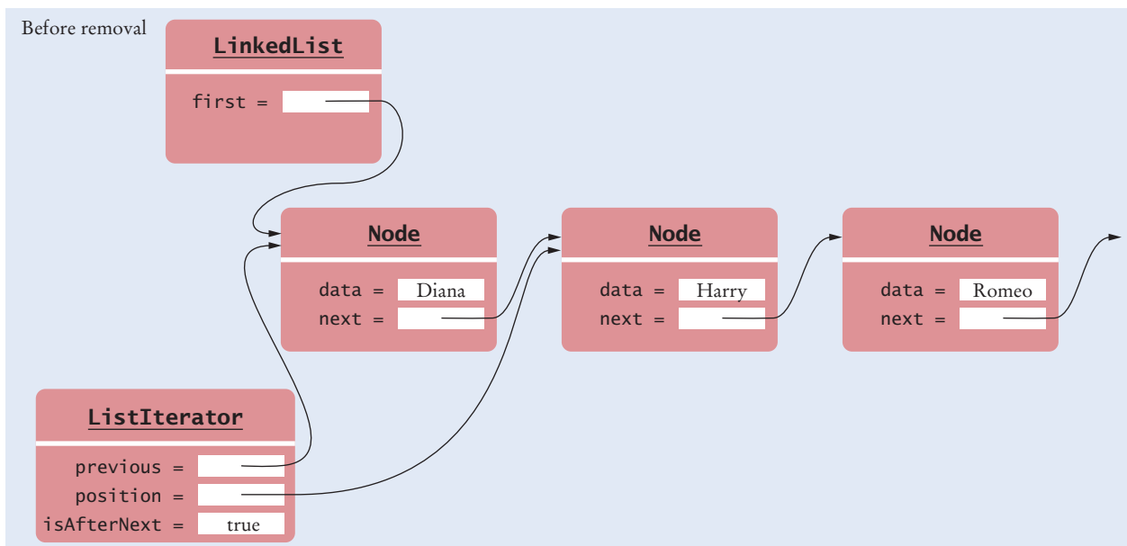
Figure 3 Removing a Node from the Middle of a Linked List
