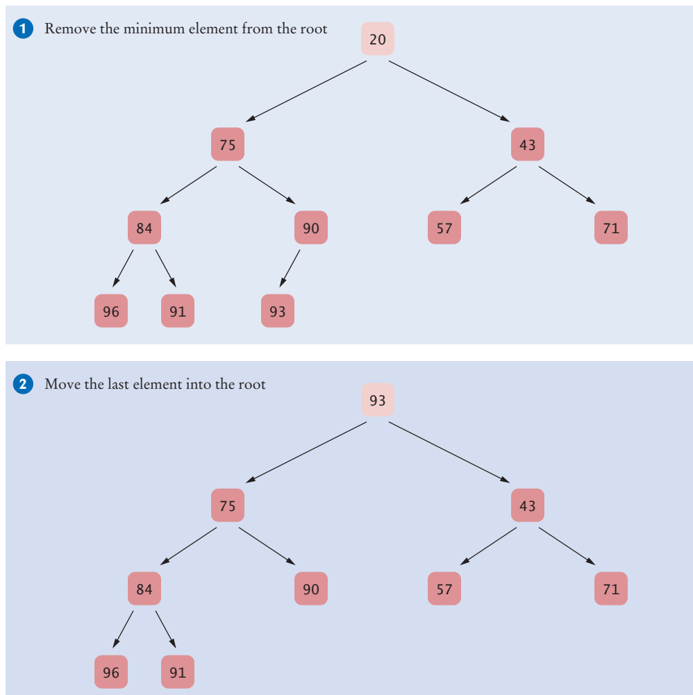
Figure 29 Removing the Minimum Value from a Heap
