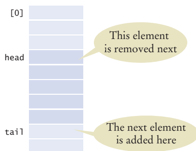
Figure 13 Queue Elements in a Circular Array
