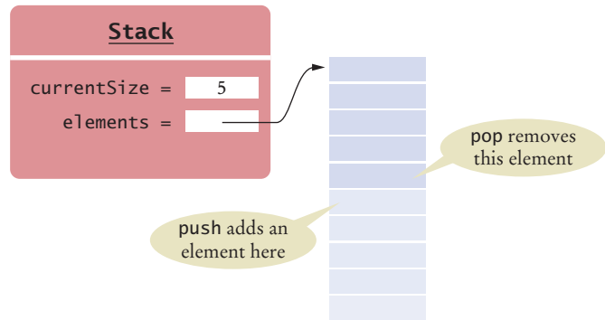
Figure 11 A Stack Implemented as an Array
