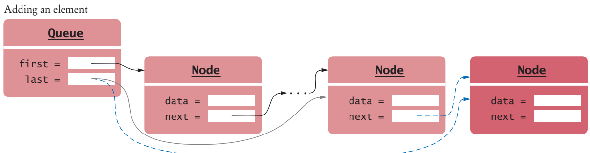
Figure 12 A Queue Implemented as a Linked List
