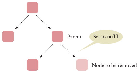
Figure 13 Removing a Node with No Children
