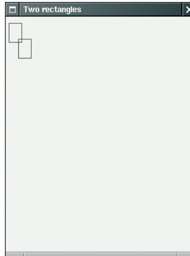
Figure 21 Drawing Rectangles
