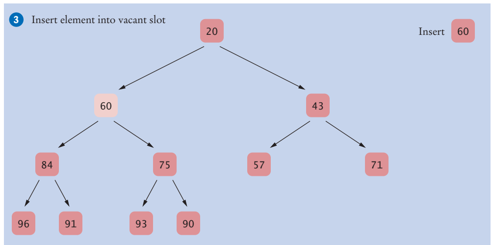
Figure 28 (continued) Inserting an Element into a Heap
