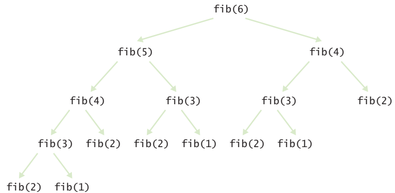
Figure 2 Call Pattern of the Recursive fib Method
