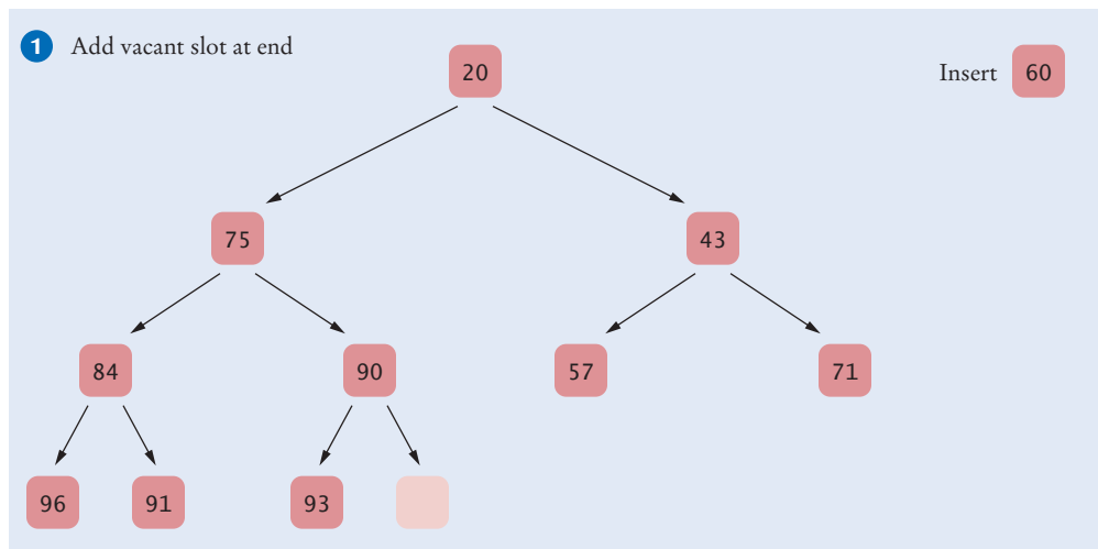
Figure 28 Inserting an Element into a Heap
