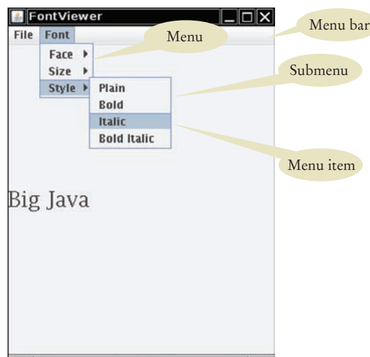
Figure 11 Pull-Down Menus
