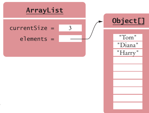
Figure 7 An Array List Stores its Elements in an Array
