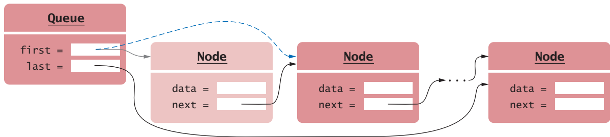
Figure 12 (continued) A Queue Implemented as a Linked List
