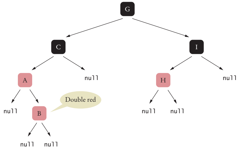
Figure 20 A Tree that Violates the “No Double Red” Rule
