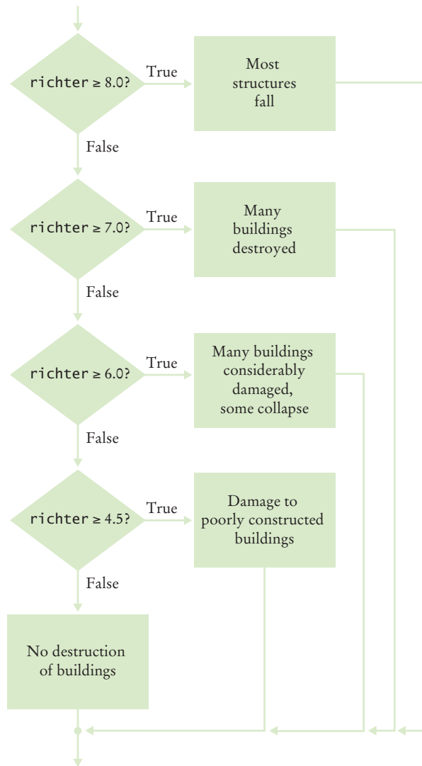
Figure 4 Multiple Alternatives
