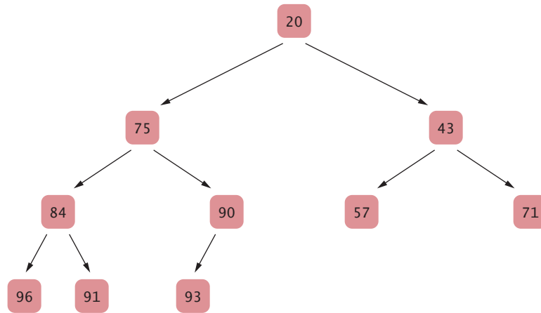
Figure 27 A Heap
