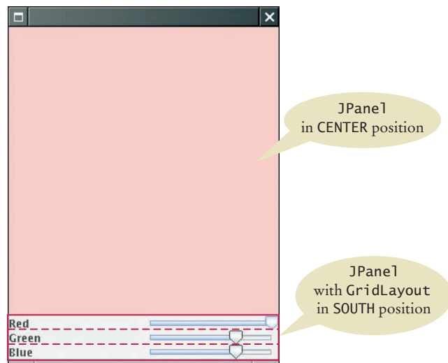
Figure 15 The Components of the Color Viewer Frame
