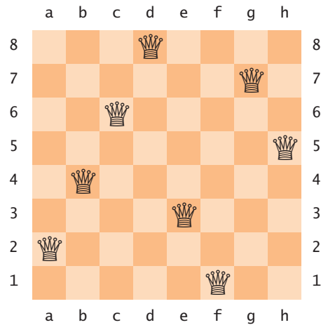
Figure 5 A Solution to the Eight Queens Problem
